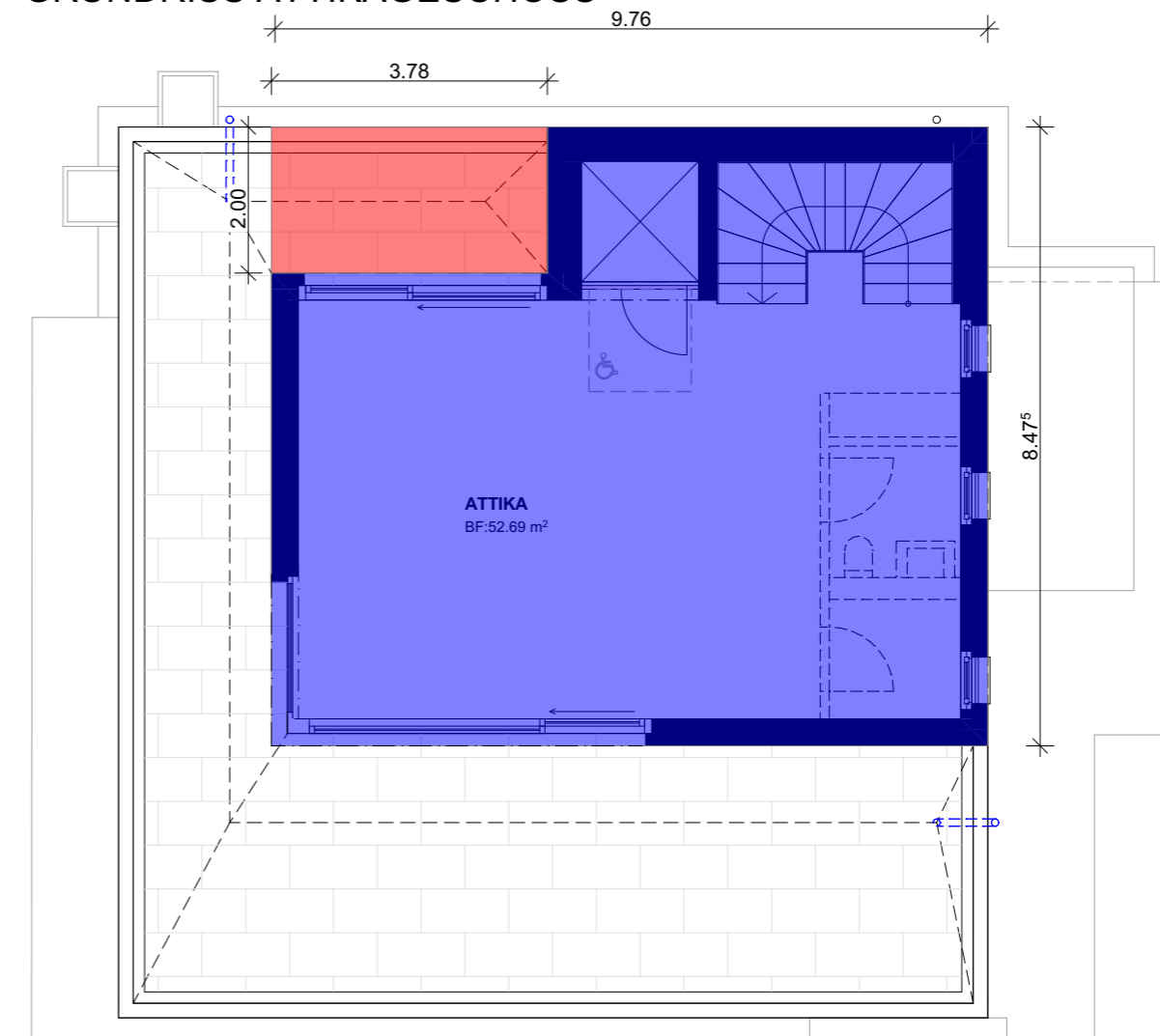
GRUNDRISS ATTIKAGESCHOSS
